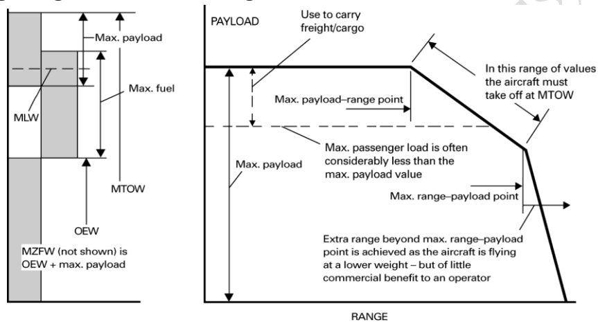
Aircraft masses and the associated payload–range diagram.
