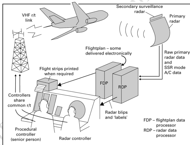
Schematic diagram of a first-generation 'automated' ATC system
